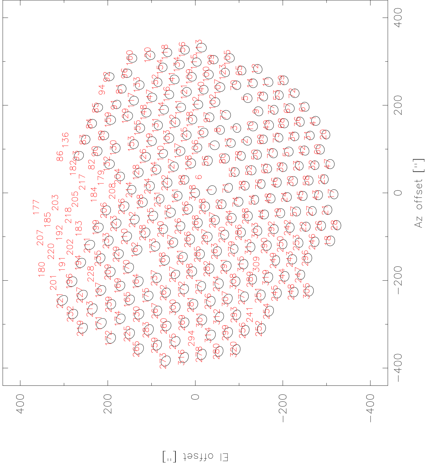
LABOCA Beam map - Scan 16527
