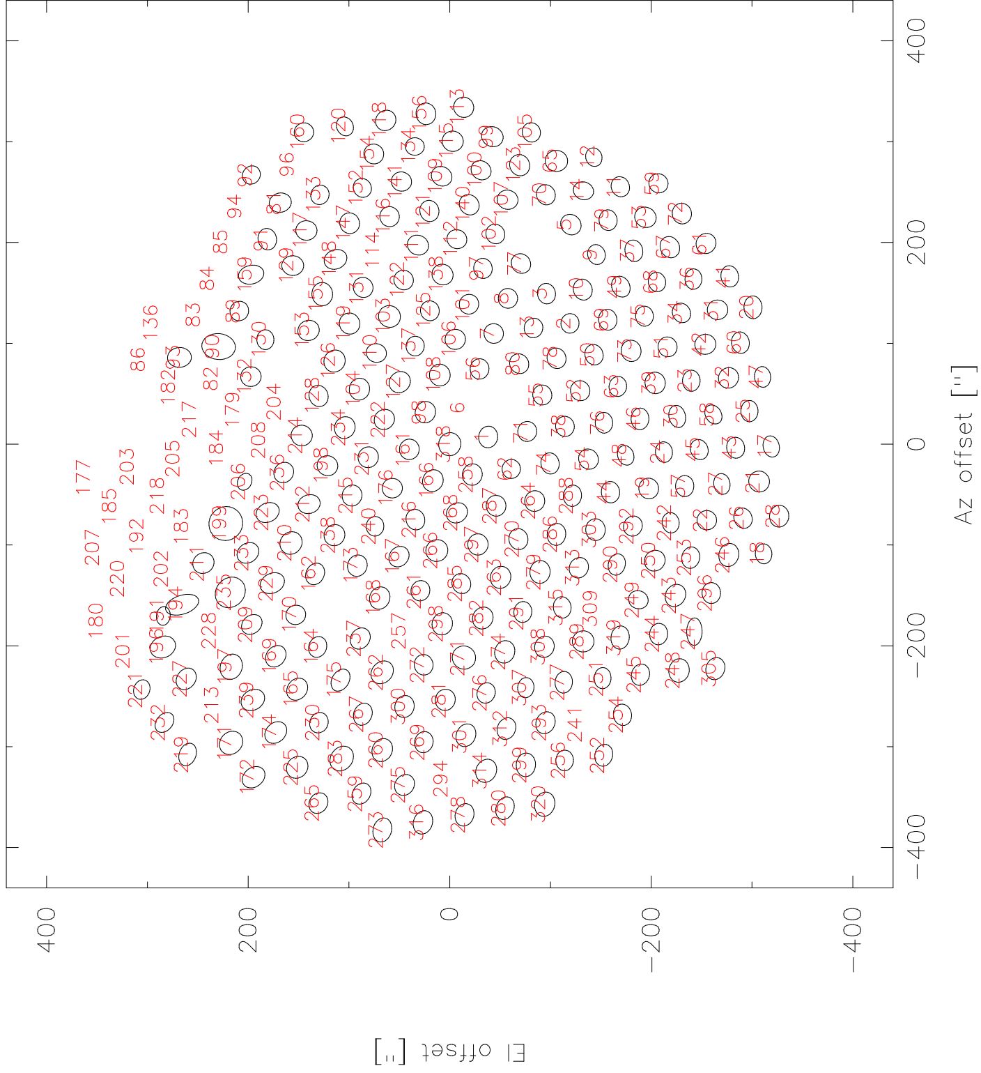
LABOCA Beam map - Scan 38096
