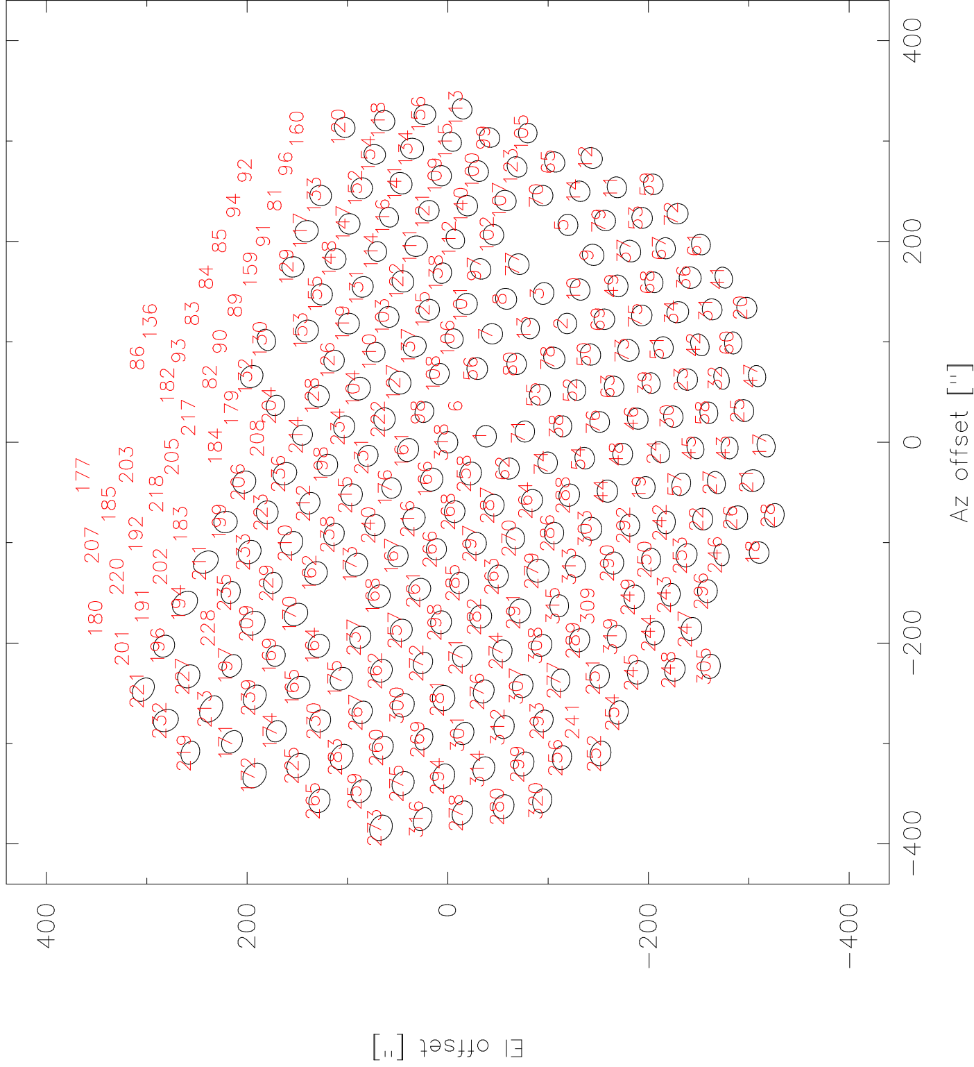
LABOCA Beam map - Scan 8643
