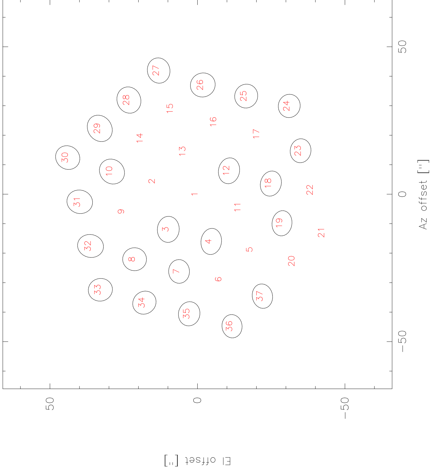
SABOCA Beam map – Scan 51773
