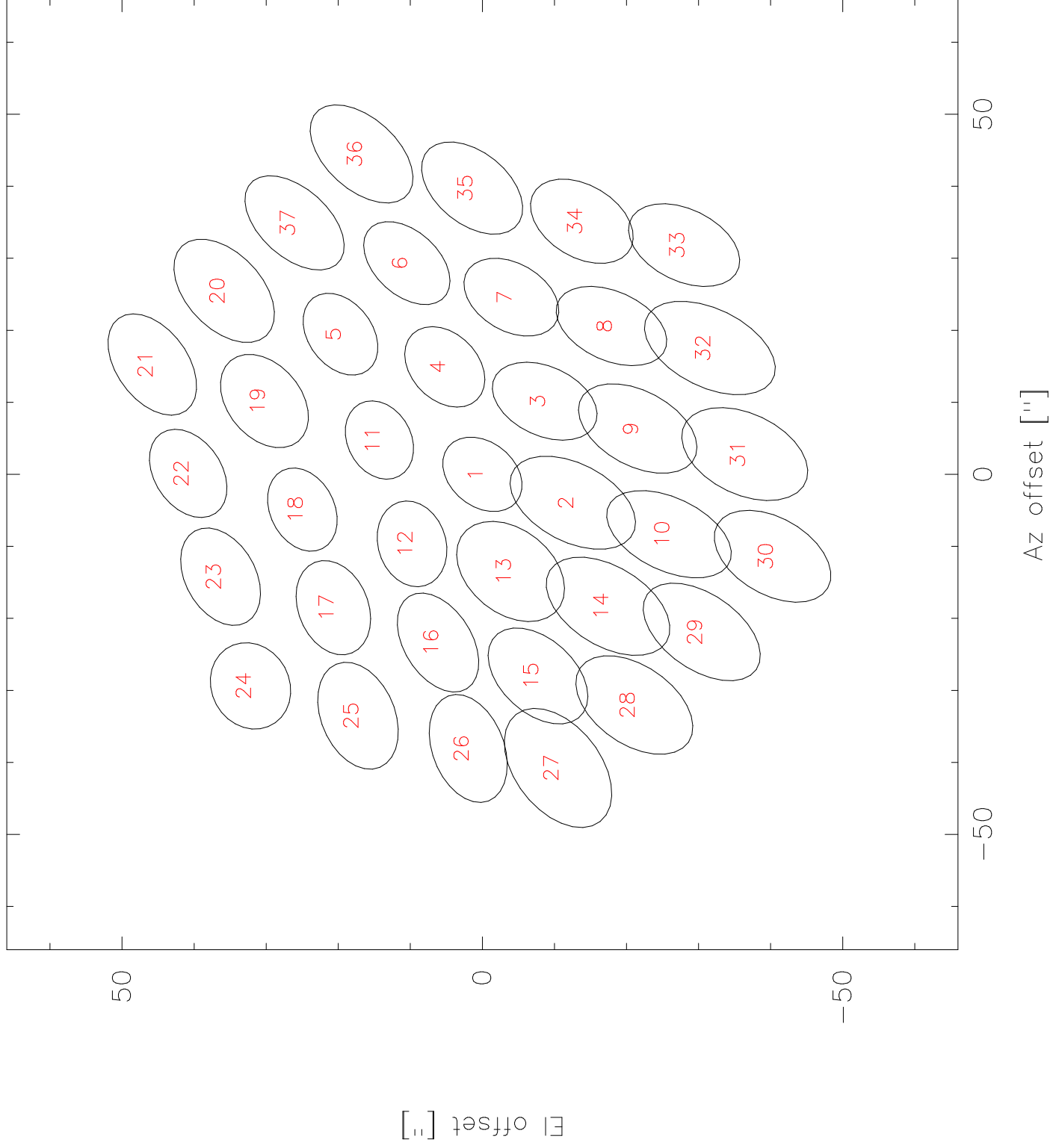
SABOCA Beam map - Scan 38437
