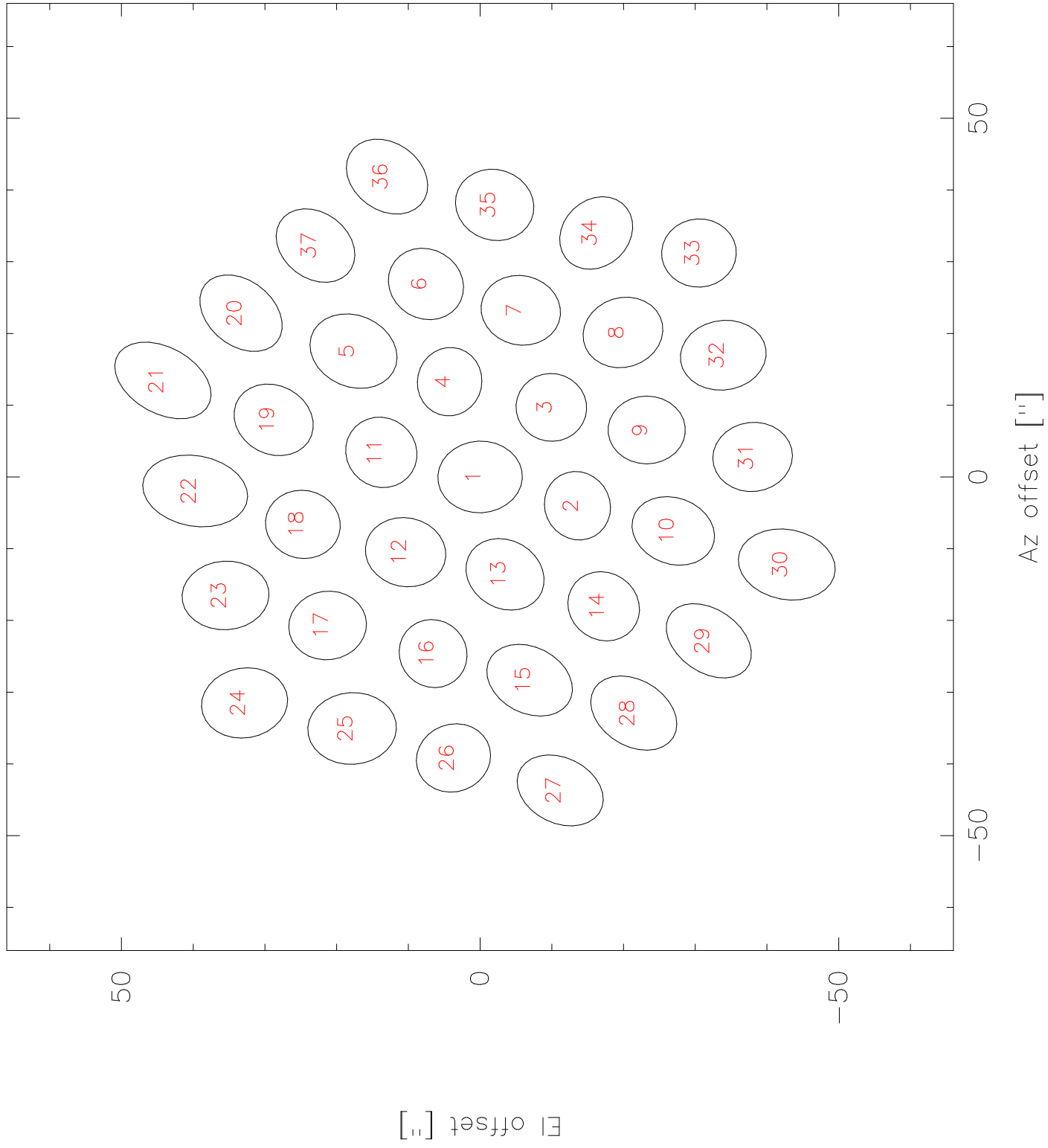
SABOCA Beam map - Scan 10054
