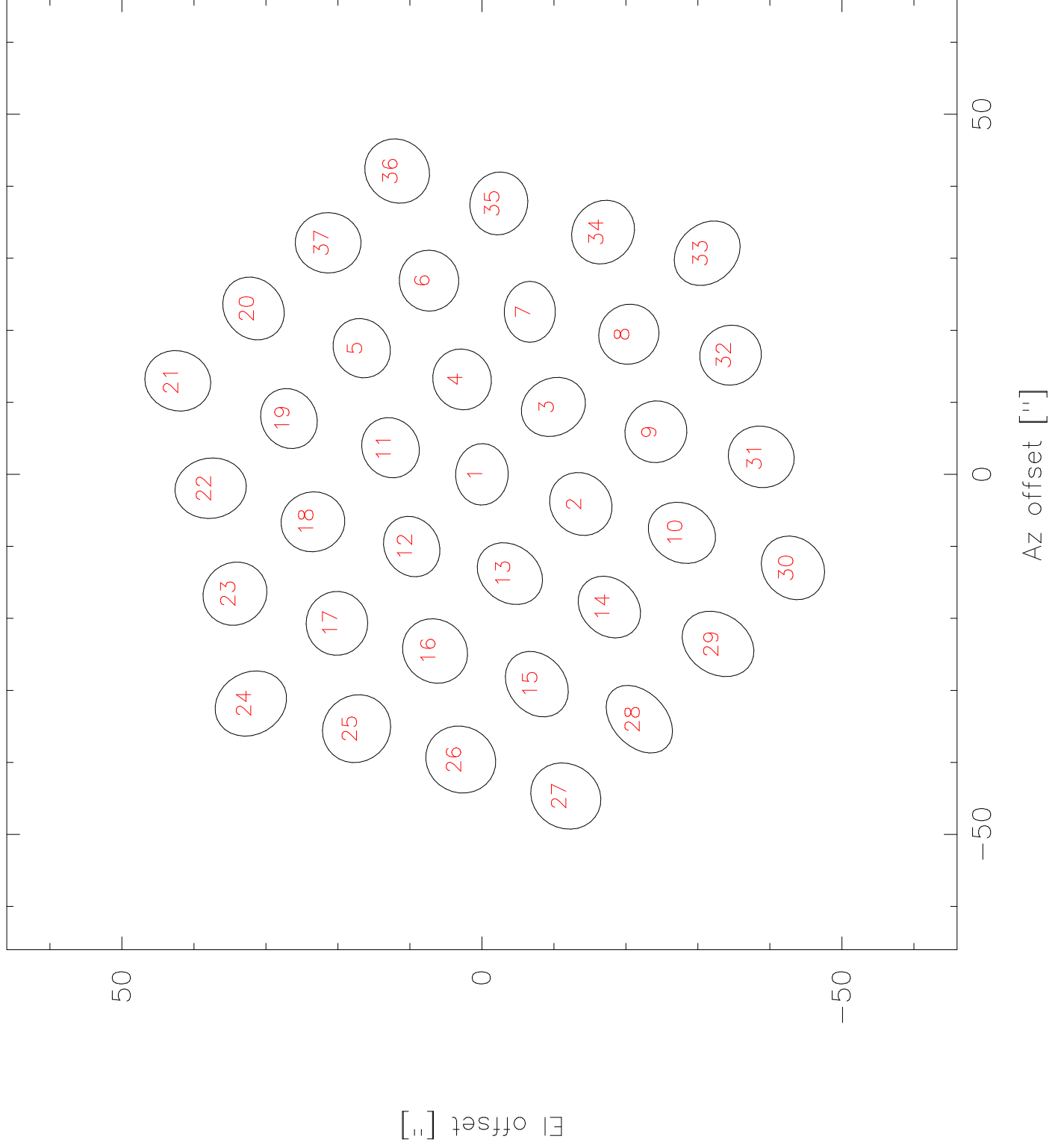
SABOCA Beam map – Scan 24044
