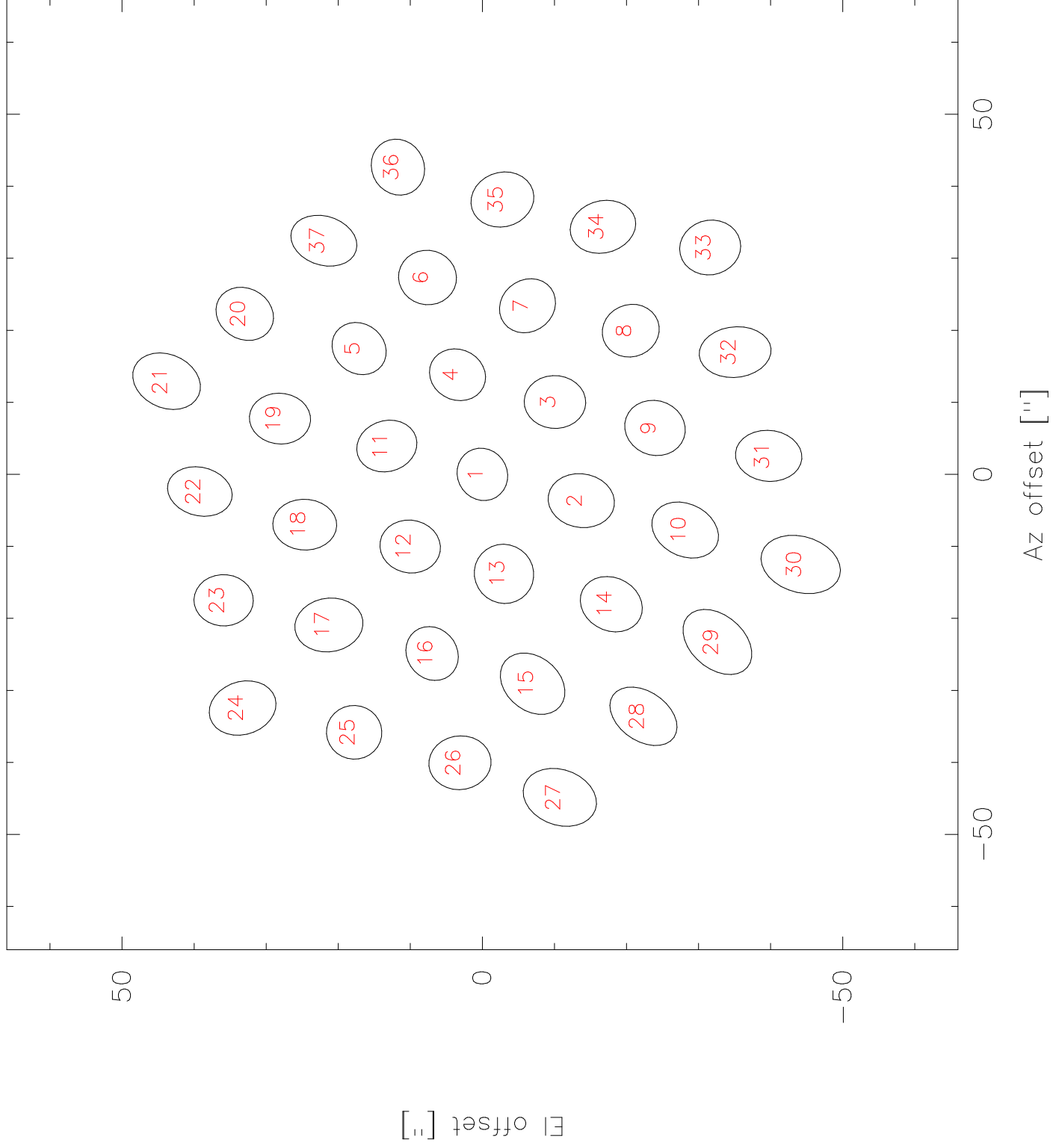
SABOCA Beam map – Scan 21457
