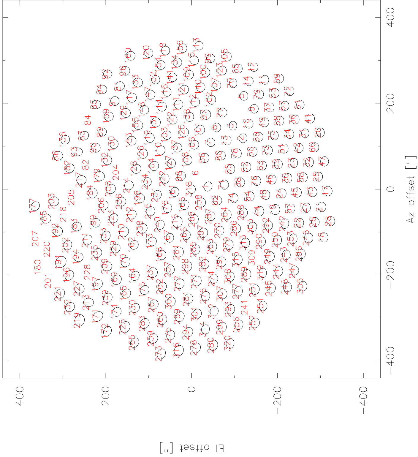
LABOCA Beam map - Scan 22335
