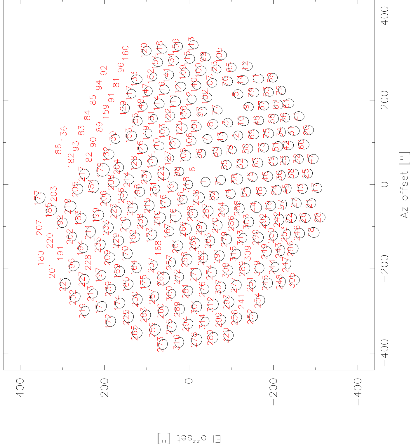
LABOCA Beam map – Scan 35493
