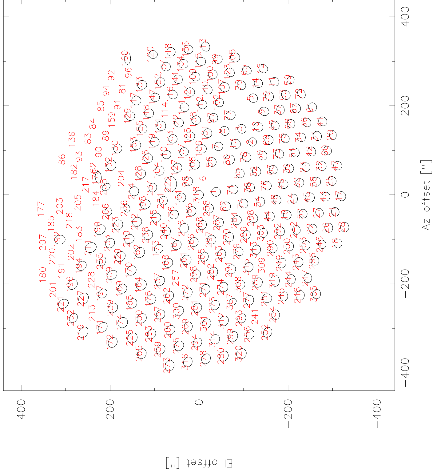
LABOCA Beam map – Scan 77888
