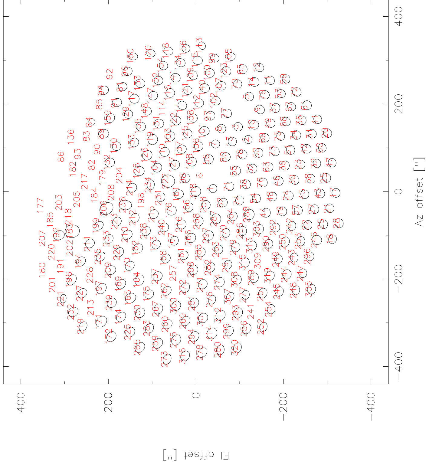
LABOCA Beam map – Scan 80078
